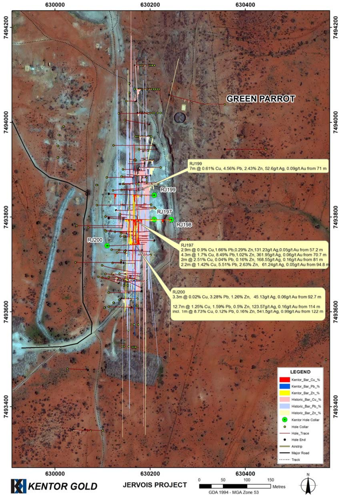
Figure 1 Green Parrot - Plan of drilling
