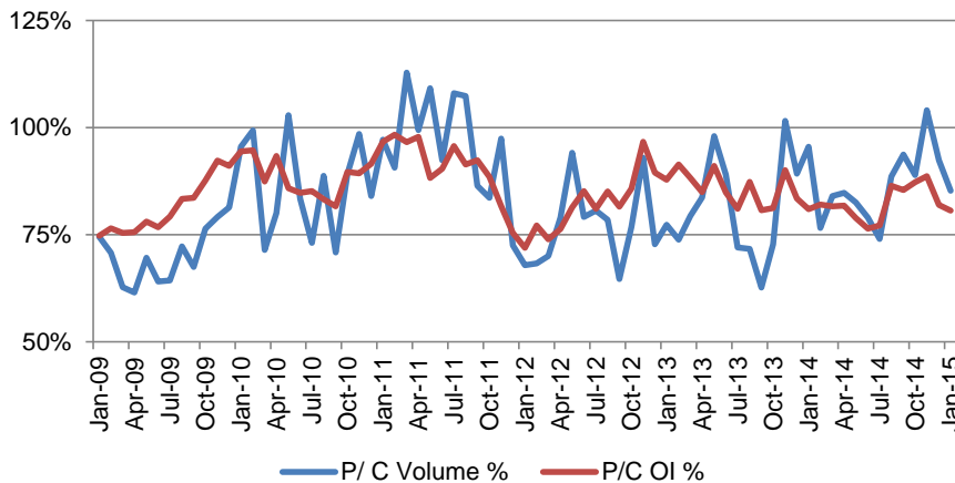
Put-Call Indicators
