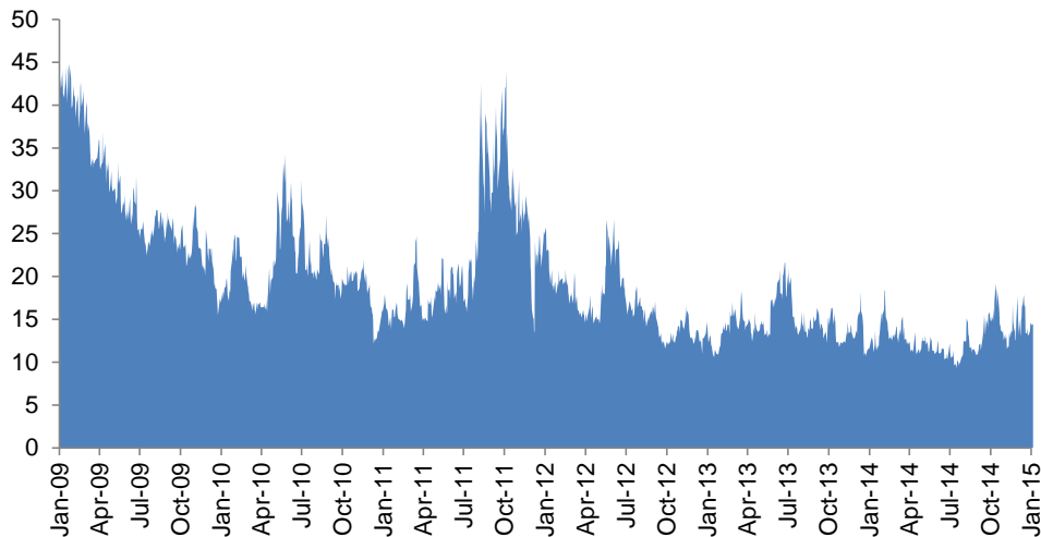
S&P/ASX 200 VIX
